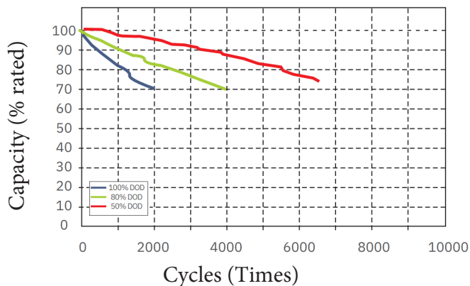
Cycle Life vs. Depth of Discharge (DOD) Discharge 0.5C / Charge 0.5C (25°C)
